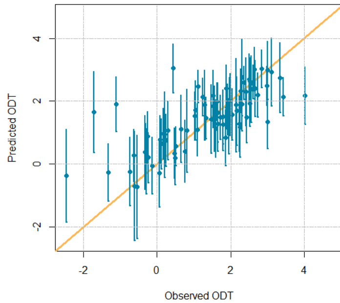
Fig. 12 Predicted values plotted against observed values for ODT for the independent test set, using the Alchemite Imputation model. Error bars on predictions represent the estimated uncertainty (one standard deviation) in each prediction
