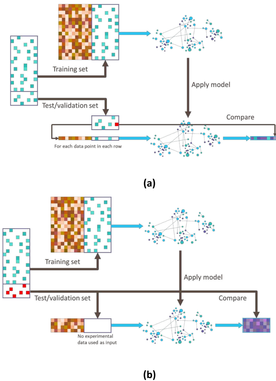
Fig. 2 The processes to build and validate imputation (a) and virtual (b) models. The training and test sets consist of rows representing different compounds. For both models, all of the experimental data for the training set (green squares) are used to train a model. For the test or validation set of an imputation model, a leave-one-out approach is used to test the accuracy of the imputation of each experimental endpoint. For a given row, one data point (red square) is omitted and the remaining experimental data (green squares) are used as input to the model. The predicted value (purple square) is compared with the held-out data point. This is repeated for each data point in each row of the test set. For the test set of the virtual model, no experimental data are used as input and the predicted values (purple squares) are compared with the experimental values in the test or validation set (red squares)
