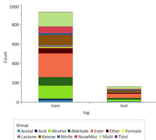
Fig. 5 Chemical composition of the training (931 compounds) and test (163 compounds) sets
