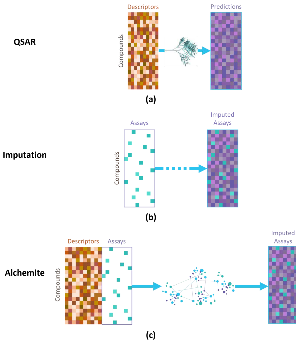
Fig. 1 A comparison of QSAR regression e.g. random forest models (a), with imputation (b) and the e.g. the Alchemite deep imputation software (c). Compound descriptors are illustrated by orange squares in a complete matrix, experimental data are shown as green squares in a sparse matrix and predicted values as purple squares
