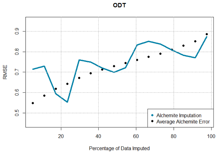
Fig. 13 Percentage of imputed values for ODT after removing the predicted values with greatest uncertainty against Root Mean Square Error (RMSE) (blue) and the average error bars from the Alchemite Imputation model for the remaining predictions are shown as black dots
