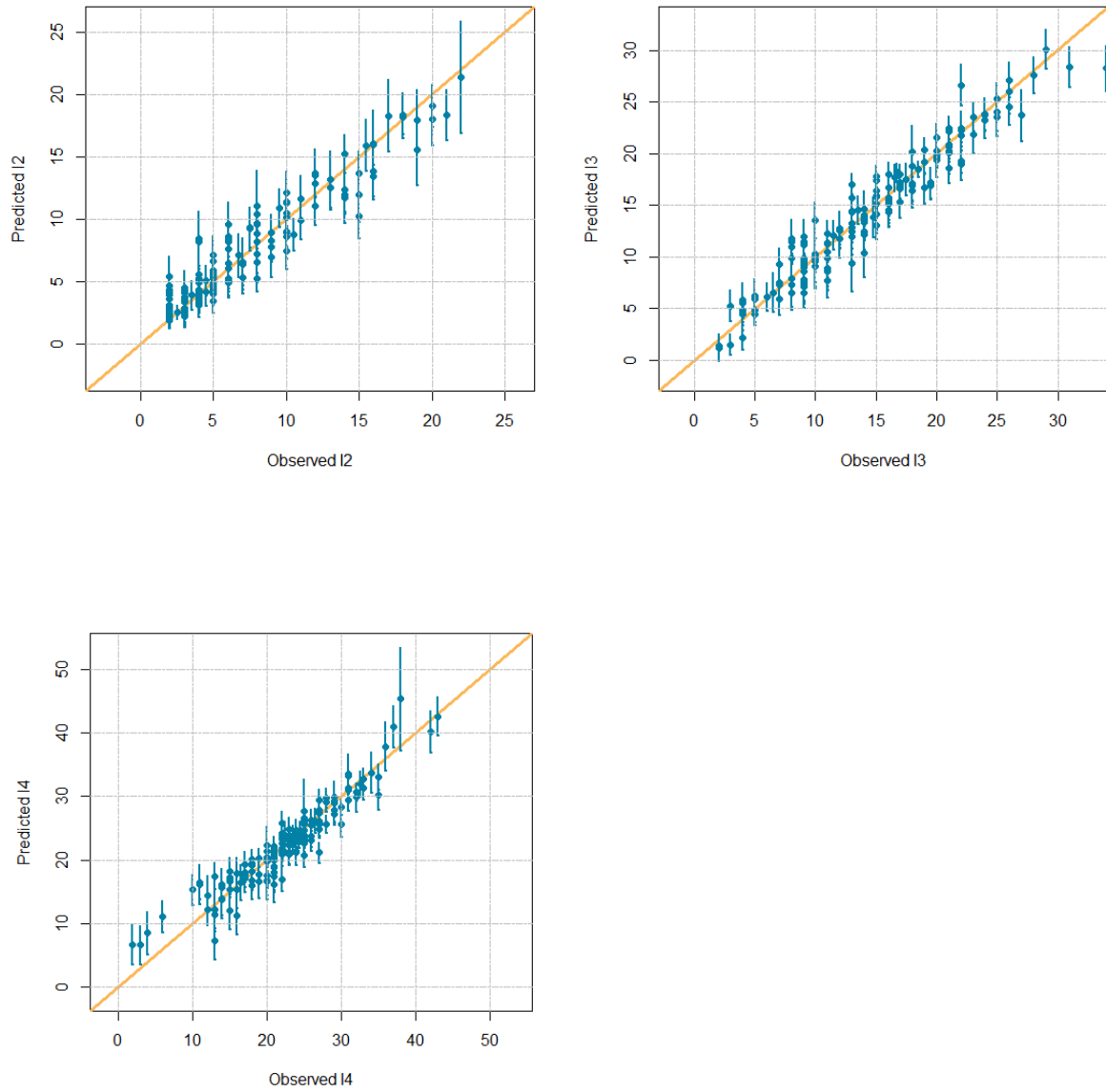
Fig. 11 Observed values plotted against imputed values for odor intensity properties, I2, I3 and I4, with error bars on predictions
