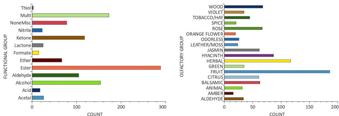
Fig. 3 Distribution of data set compounds across chemical classes and odor categories
