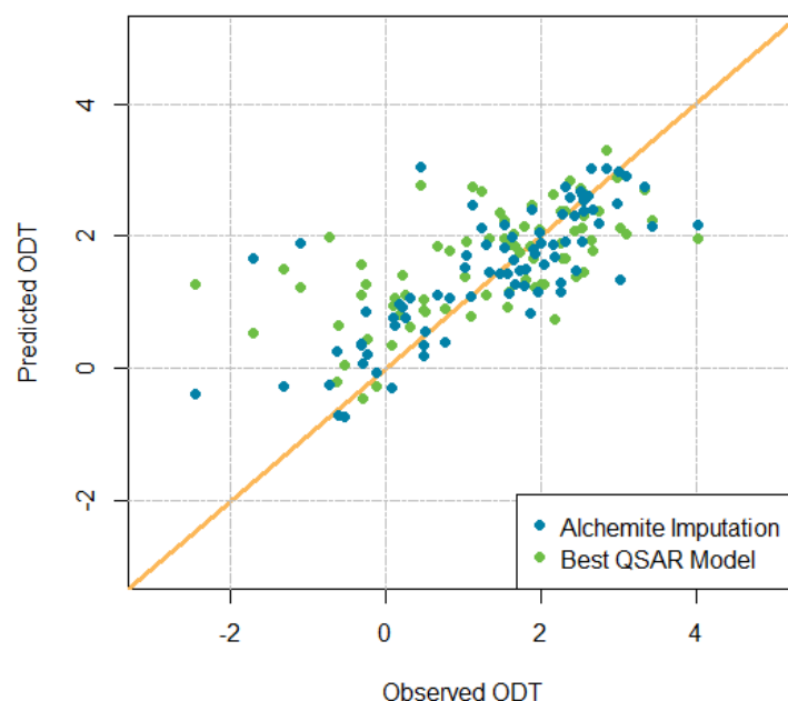
Fig. 10 Predicted values plotted against observed values for ODT for the independent test set, using the Alchemite Imputation model (blue) and the best QSAR model (green)
