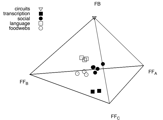
FIG. 3: Clustering signature tetrahedron with the positions of the 16 networks of five different types (see legend). K-means clustering separates these classes perfectly. The tetrahedron corresponds to the feed-forward subspace of the normalized clustering signatures, i.e. ( \tilde{C}_{FFA} , \tilde{C}_{FFB} , \tilde{C}_{FFC} ), so that the FB vertex corresponds to (0, 0, 0), and the FF_A , FF_B and FF_C vertices correspond to the (1, 0, 0), (0, 1, 0) and (0, 0, 1) points respectively. If a network only has feedback loops and no feed-forward loops (such as the electric circuits studied in this paper), it will be located at the FB vertex. Conversely, a network without any feedback loops will be located at the base of the tetrahedron. The location of a network relative to the FF_A , FF_B and FF_C vertices signifies the relative dominance of the given node roles (see Figure 2). As an illustration, consider the transcription networks (black squares) which have a k-means centroid of (0.145, 0.232, 0.622). The normalization implies that \tilde{C}_{FB} = 1 - 0.145 - 0.232 - 0.622 = 0.001 so that these networks will be located at the base of the tetrahedron. The FF_A component is also negligible, so that the networks lie on the edge opposite the FF_A vertex, slightly closer to FF_C than FF_B because the FF_C component is larger.
