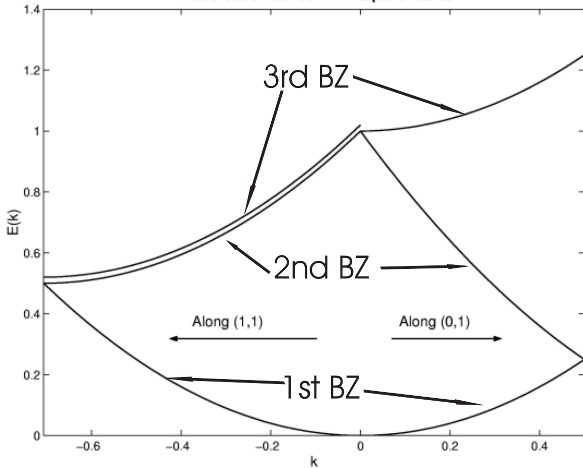
Free electron bands in 2D square lattice
