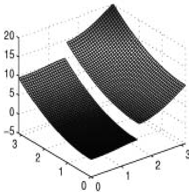
Both bands in extended zone scheme
