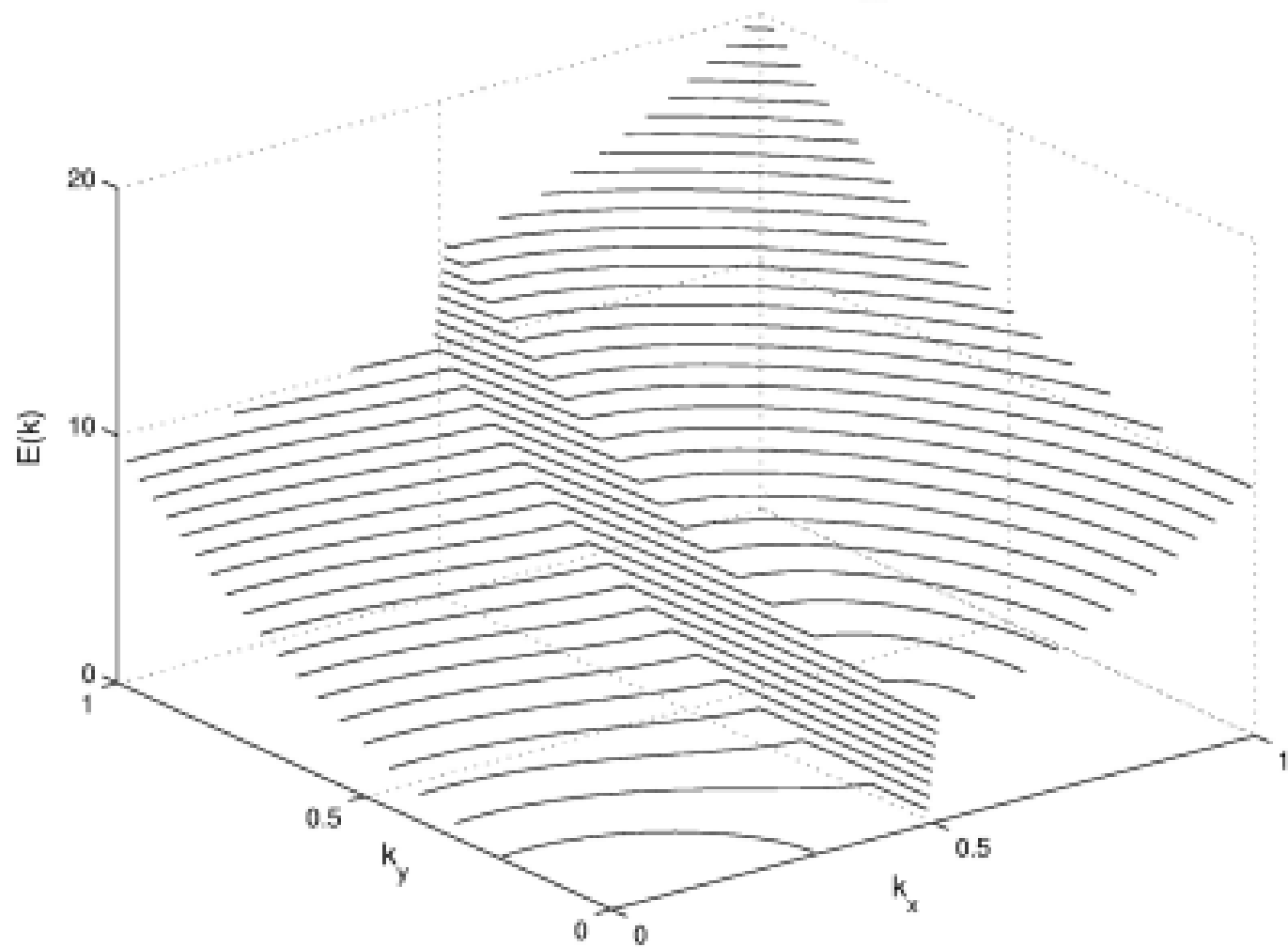
Contours of constant energy
