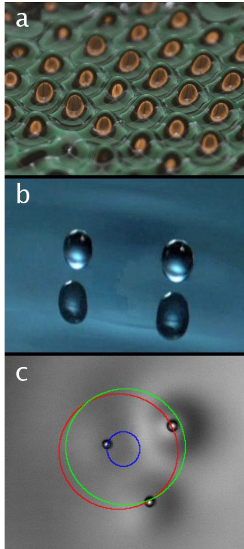
Figure 1: a) Millimetric Faraday waves are generated on the surface of silicone oil by driving it vertically in a periodic fashion above the Faraday threshold. b) A pair of droplets (diameter 2 mm) on the surface of silicone oil, above the bouncing threshold but below the Faraday threshold. The droplets communicate through their wave fields, locking into phase a fixed distance apart. c) Three walking droplets lock into a collective orbit. All orbits are counterclockwise, the largest being 8 mm in diameter.
