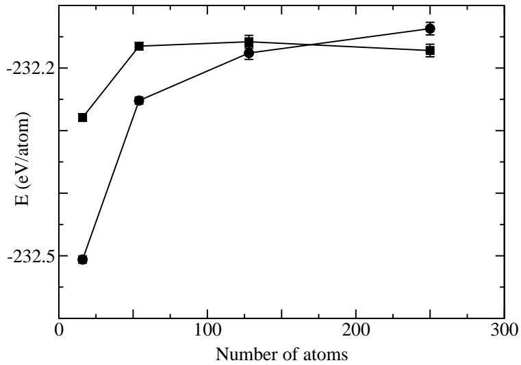
Figure 2: The VMC energy per atom for MgO in the rock-salt structure with a volume per atom of 9.06 Å 3 as a function of the number of atoms in the repeating cell, using both the Ewald interaction (circle) and the MPC interaction (squares).
