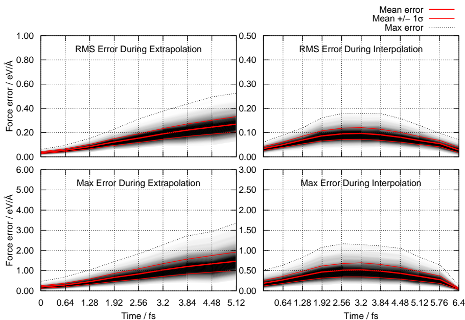
Figure 4.13: As in Fig. 4.12, but the test system is that shown in Fig. 4.9b, again at a temperature of 2000 K, with MD timestep \Delta t = 0.64 fs and N_{\text{interp}} = 10 . The linear spring adjustable potential with two body springs only was used. The QM force model was the DFTB method of Frauenheim et al. [91].
